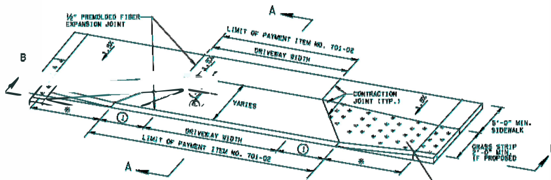
TYPE "A" DRIVEWAY ACROSS SIDEWALK WITH GRASS STRIP
